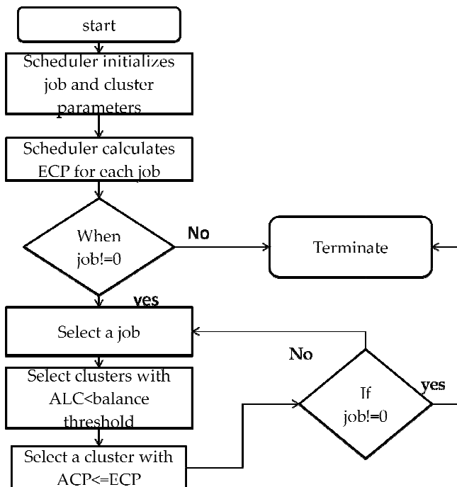
Fig 4.1: flowchart for EHLBA
