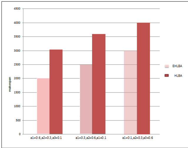
Fig 5.1- Graph showing makespan for weighted values in EHLBA and HLBA
