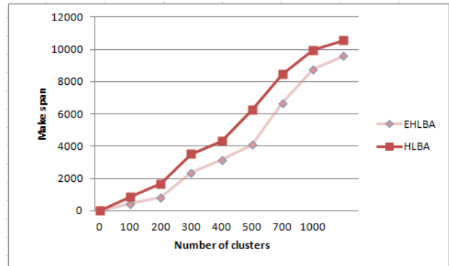
Fig 5. 2- Graph showing makespan for HLBA and EHLBA
